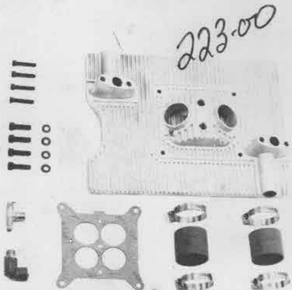
05-3040 DUAL TURBOCHARGER MOUNTING ADAPTOR
