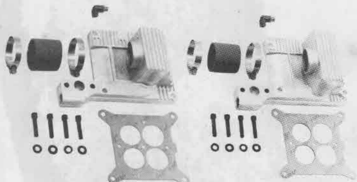
SINGLE TURBOCHARGER MOUNTING ADAPTOR 05-2440 05-2540
