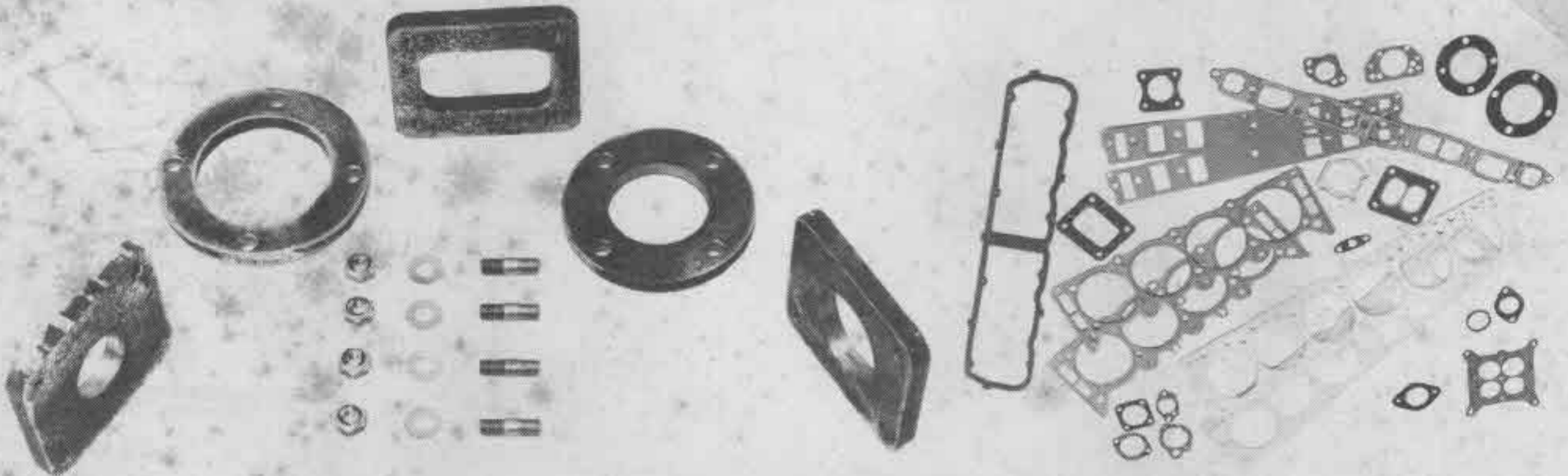
ASSORTED FLANGES AND GASKETS TO ASSIST IN 'ONE-OFF' INSTALLATIONS
